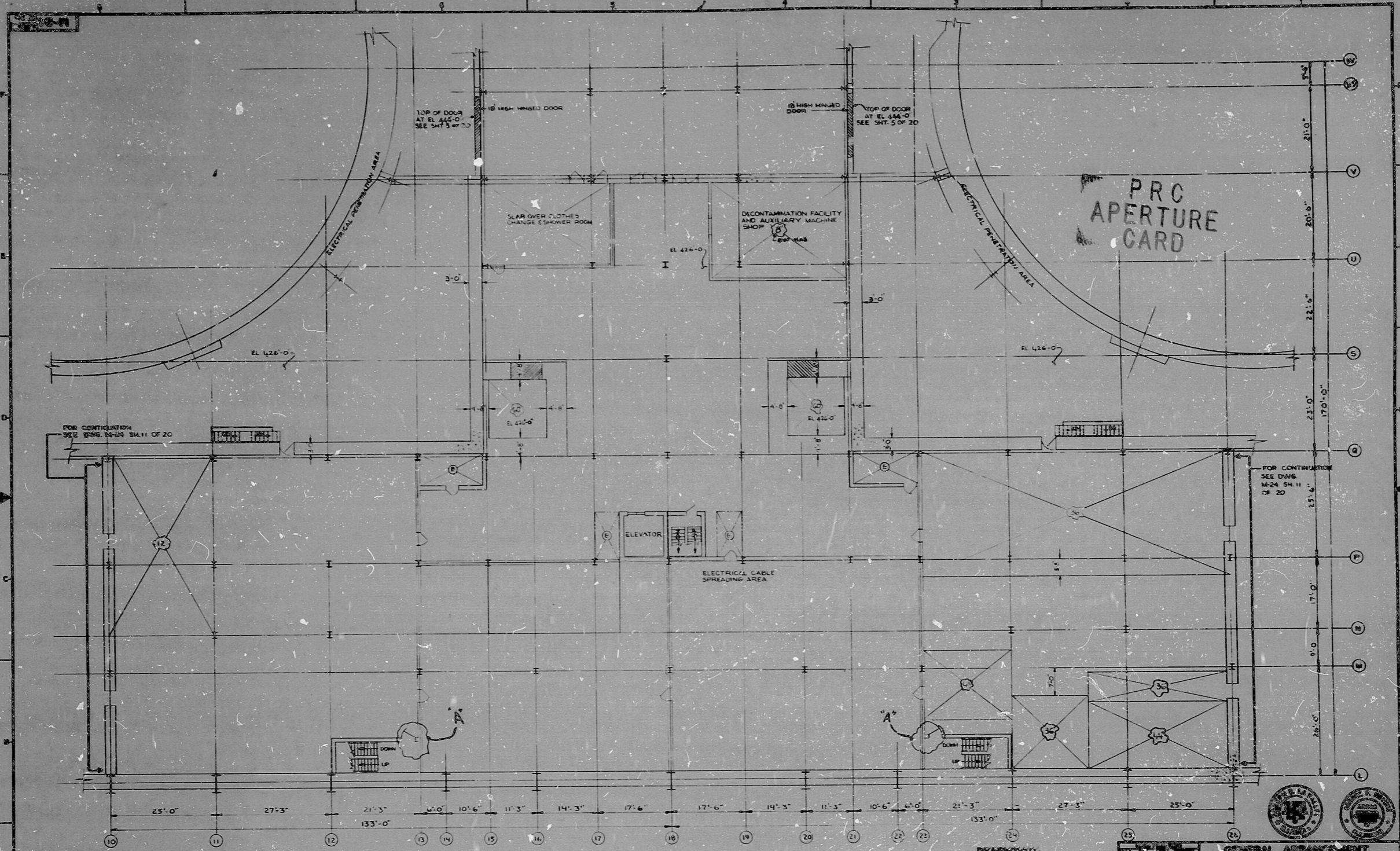
PLAN EL. 439'-0"
