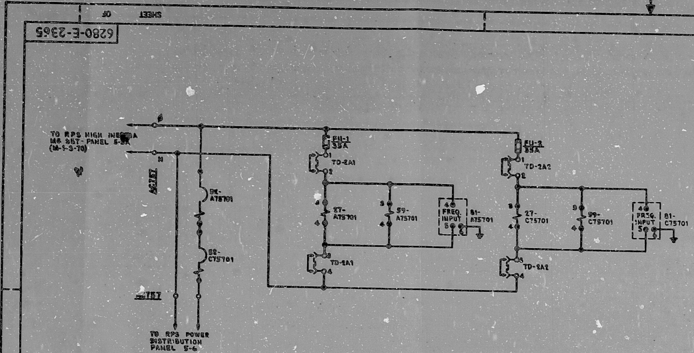
RPS BREAKER PANEL 2AC757 RPS BREAKER PANEL 2BC757 SIMILAR
