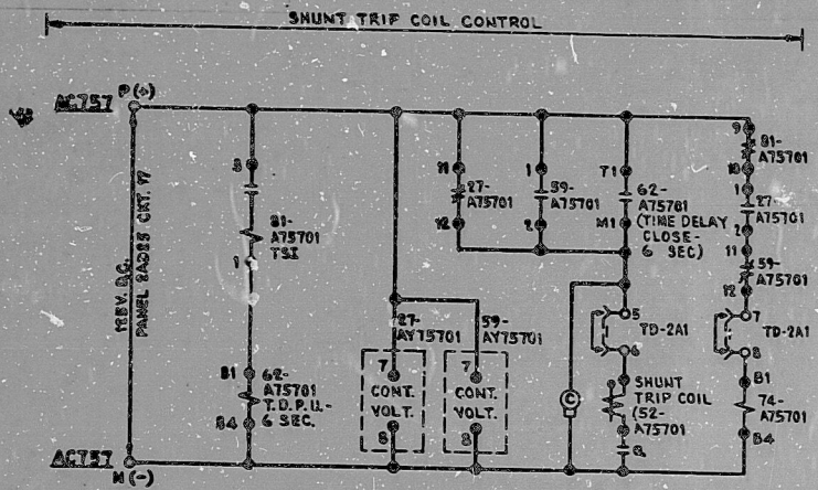
SCHEME 2AY75701 TYPICAL FOR 2BY75701 TYPICAL FOR UNIT 3
