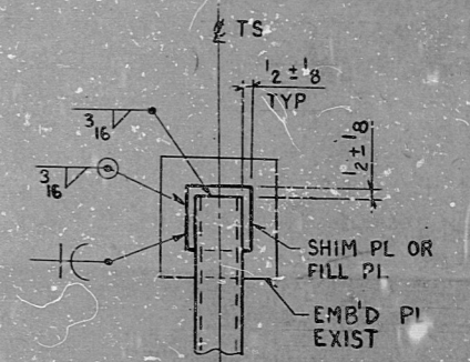
SECT DM
