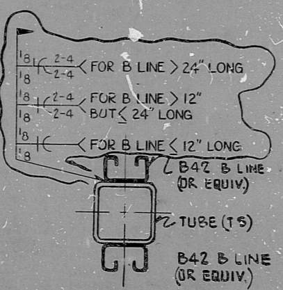
DETAIL FA2
