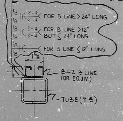
DETAIL FA1
