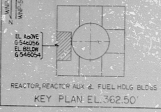
REACTOR, REACTOR AUX & FUEL HLG BLDGS KEY PLAN EL.362.50'
