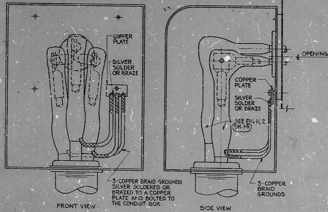
FIG. 4 TERMINATION OF 5KV CABLE SHIELDS IN MOTOR CONNECTION BOX
