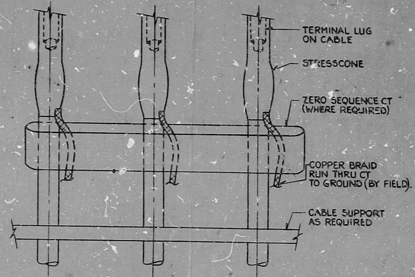
FIG. 5 TERMINATION OF 5KV IN 15KV CABLE SHIELDS IN SWITCHGEAR ENCLOSURES WITH BUS BARS
