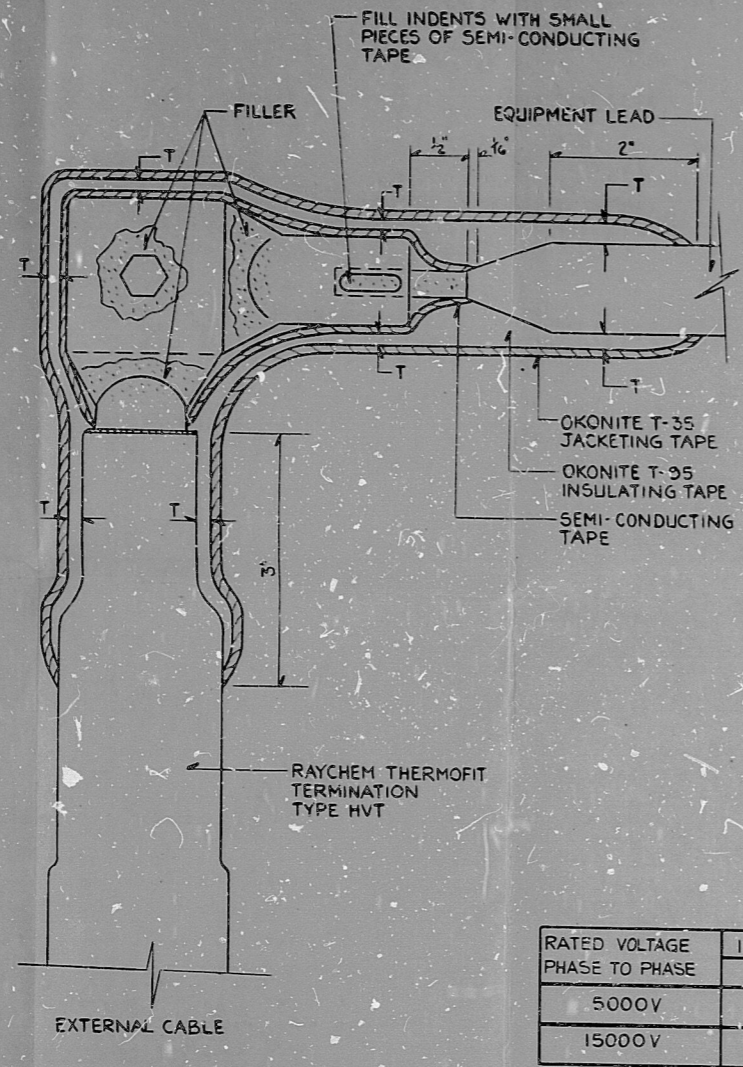
FIG. 1 5 KV CABLE CONNECTION TO MOTOR LEAD
