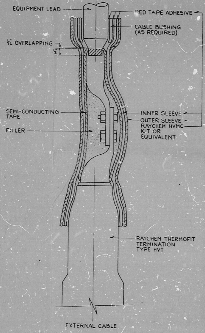
FIG. 2 5 KV CABLE CONNECTION TO MOTOR LEAD
