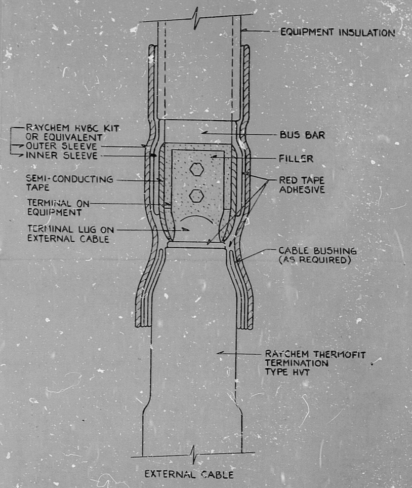
FIG. 3 5 KV & 15KV CABLE CONNECTION TO BUS BAR (90° AND STRAIGHT CONNECTION)
