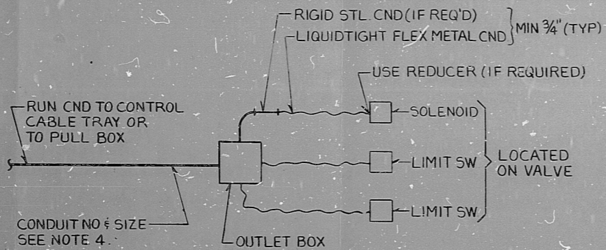
PHYSICAL CONNECTION AT VALVE
