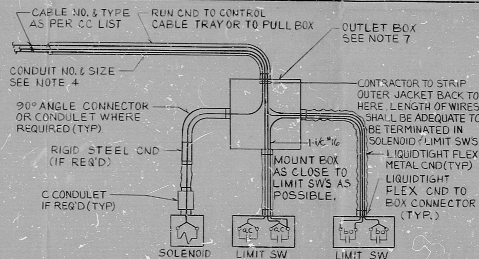
PHYSICAL CONNECTION AT VALVE
