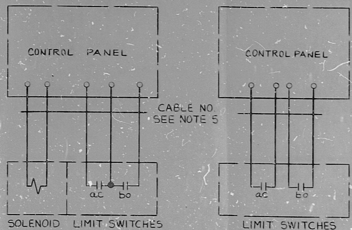
TYPICAL CWD PRESENTATION
