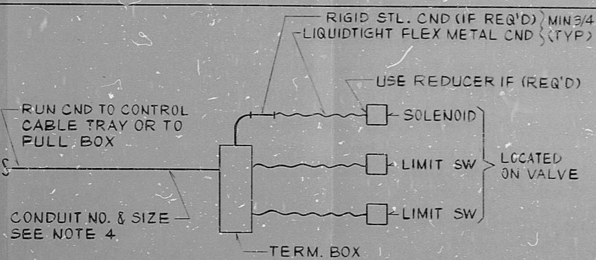
PHYSICAL CONNECTION AT VALVE
