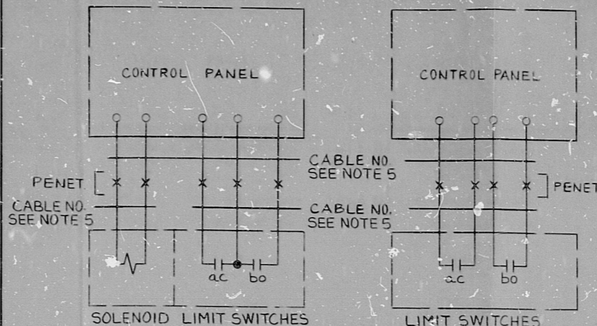
TYPICAL CWD PRESENTATION
