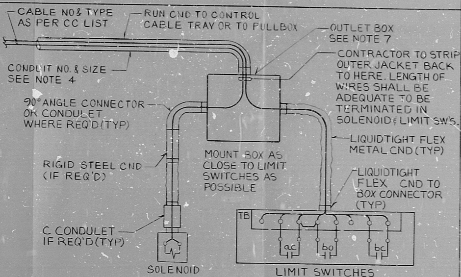
PHYSICAL CONNECTION AT VALVE
