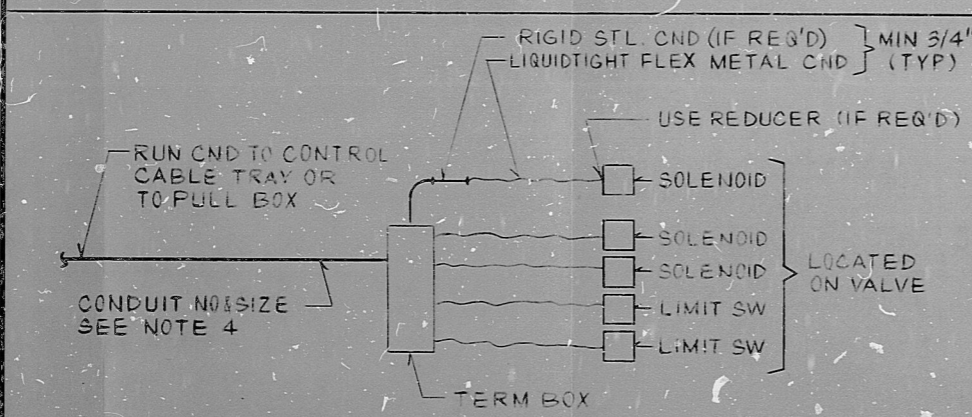
PHYSICAL CONNECTION AT VALVE
