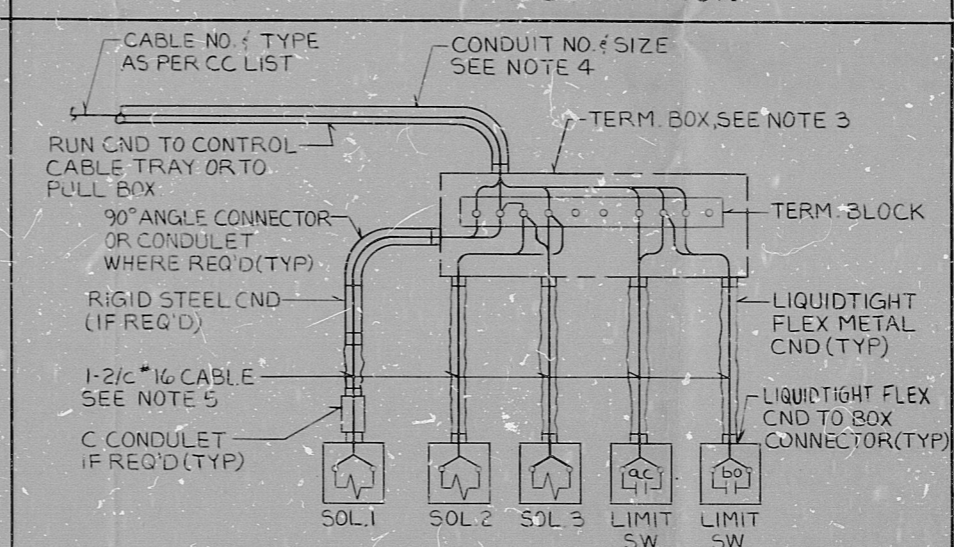
PHYSICAL CONNECTION AT VALVE
