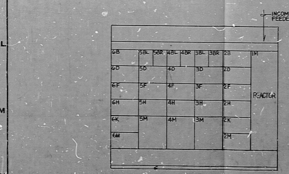
MCC B235 (FRONT VIEW)
