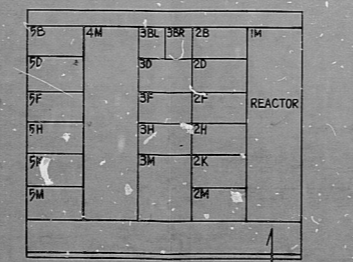
MCC B241 (FRONT VIEW) (OUTDOOR UNIT)
