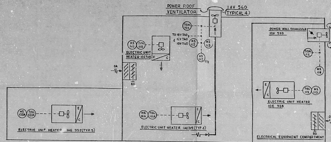
CIRCULATING WATER CHLORINATION AND ACID FEED ENCLOSURE
