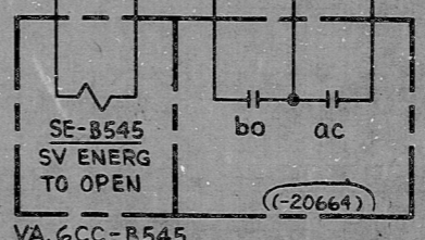
VA.GCC-B545 BORIC ACID CONCENTRATOR INLET
