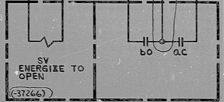
SG2 HOT LEG SAMPLE ISOLATION VA 2BD-VS090SA
