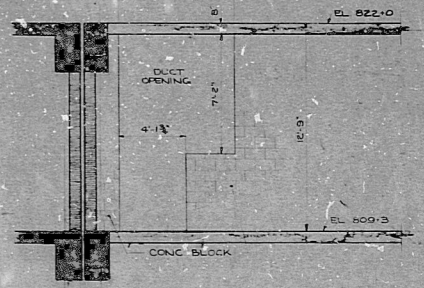
3 ELEVATION SCALE 1/4" = 1'-0"
