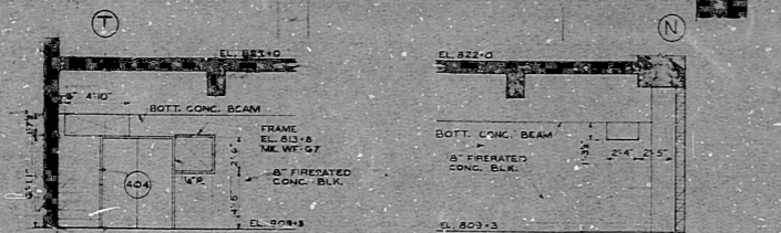
1 ELEVATION COL LINE 73 SCALE 3/16" = 1'-0" 2 ELEVATION COL LINE 73 SCALE 3/16" = 1'-0"
