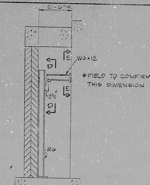
SECTION C SCALE 3/8"-1'-0" SK-C-181
