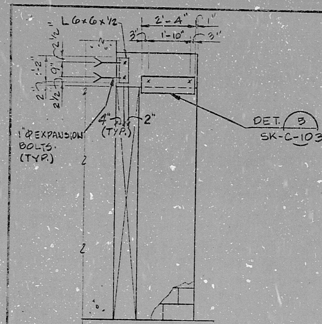
ELEVATION-LOOKING NORTH SCALE 3/8"-1'-0"
