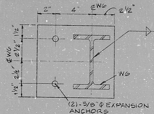
SECTION E SCALE 3"-1'-0"
