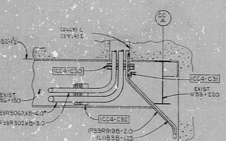
SECTION 4-4 SCALE 1/2"=FO'
