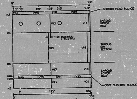
SHROUD SURFACE DEVELOPMENT
