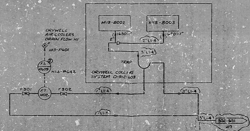
DRYWELL AIR COOLER LEAK DETECTOR (NON-SAFETY RELATED)
