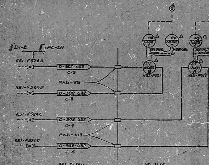
RCIC STEAM SUPPLY LEAK DETECTOR
