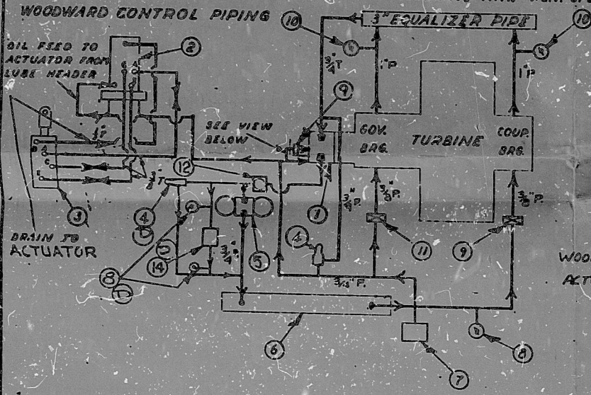
OIL PIPING DIAGRAM
