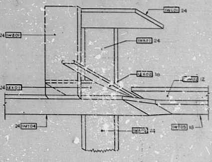
ISOMETRIC VIEW SECTION T-T SCALE: 1" = 2'-0"
