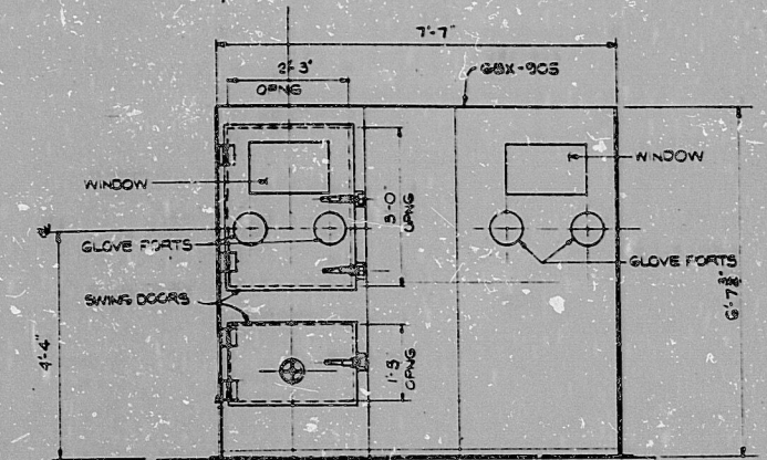
GLOVEBOX ELEVATION 1/2" = 1'-0"
