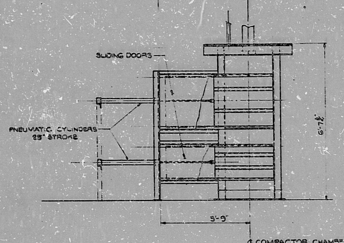
VIEW D 1/2" = 1'-0"
