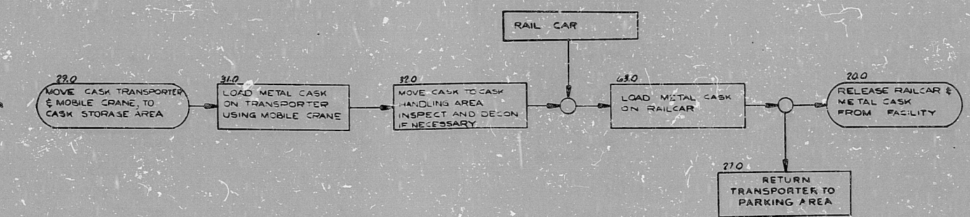
TRANSPORTABLE METAL CASK RETRIEVAL
