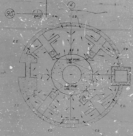
FLOOR DRAINAGE PLAN
