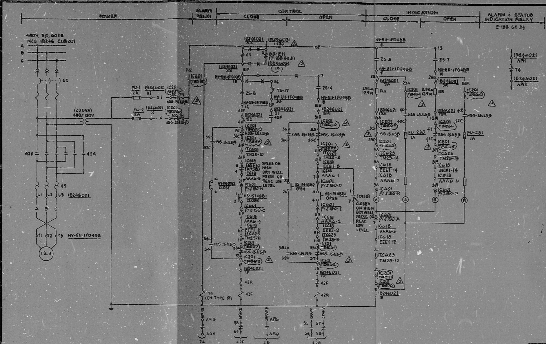
RHR HX SHELL SIDE BYPASS VALVE HV-EII-1F048B SCHEME NO. 103004 REF SH 10
