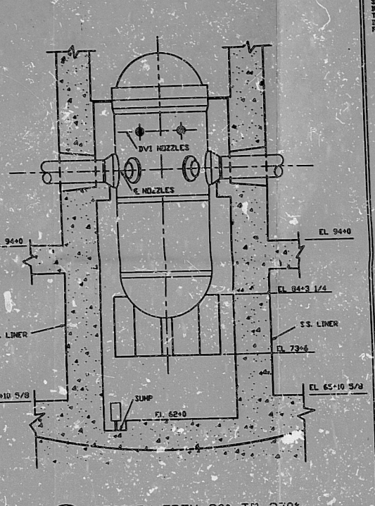
C SECTION FROM 90° TO 270°
