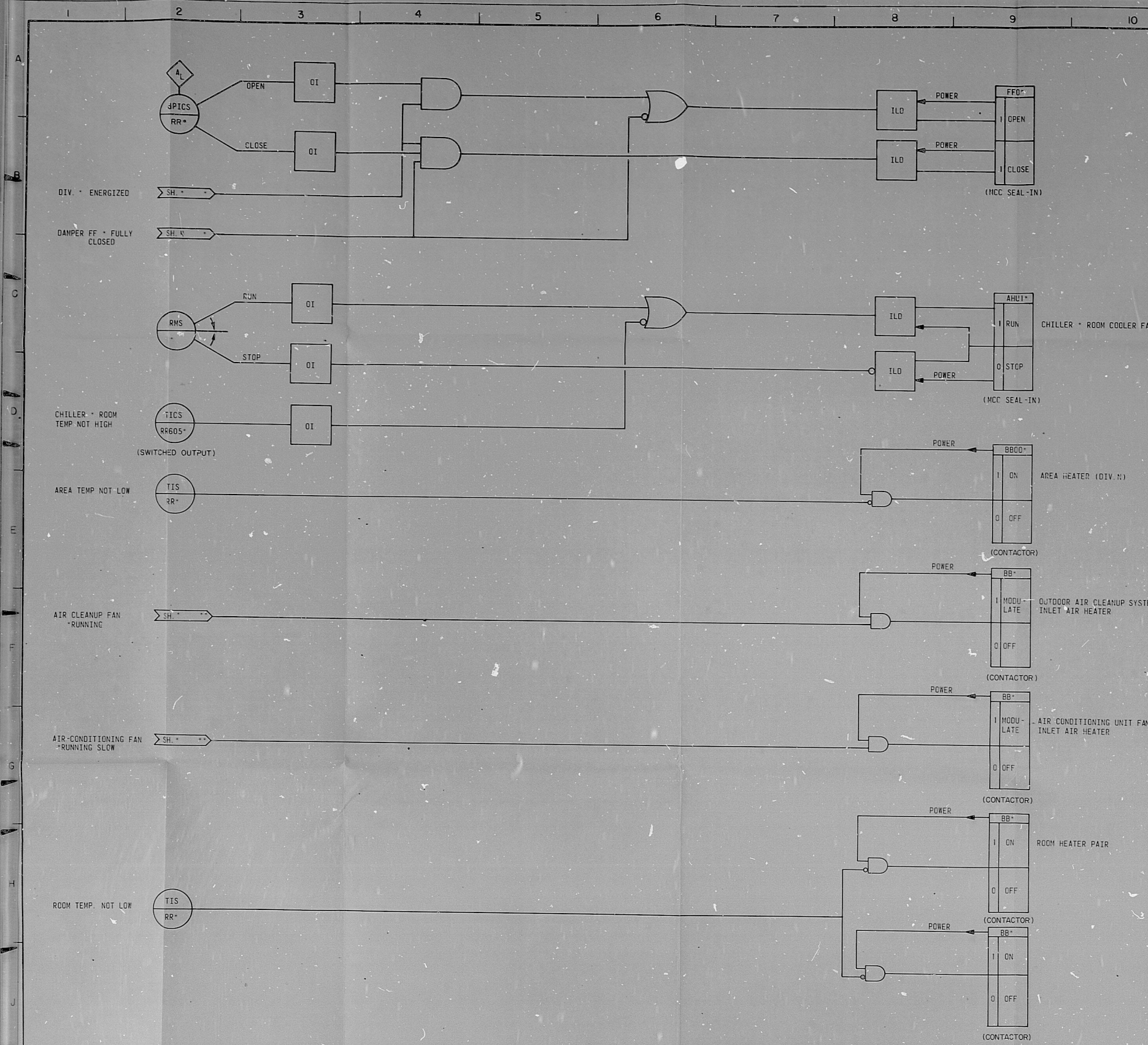
*TYPICAL FOR DAMPERS AS PER TABLE
