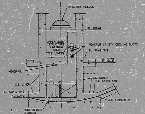
A SECTION THRU MAVED CHASE GEO-11
