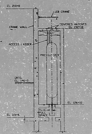
B SECTION THRU PRESSURIZER GEO-11
