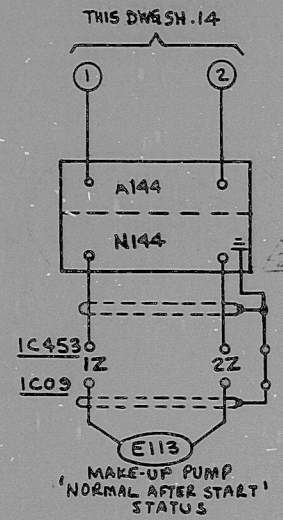
PLANT STATUS INDICATION-MAKE-UP PUMP IP-58A SCHEME INMU106 S.U. DESIG. 1-BQC
