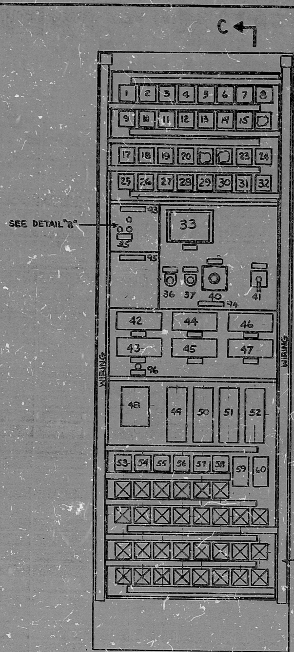
SECT B-B RELAY RACK LAYOUT (FRONT VIEW) SCALE: 1 1/2" = 1'-0"
