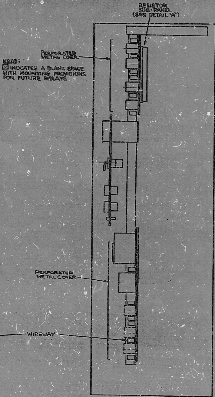
SECT C-C RELAY RACK CROSS-SECTION
