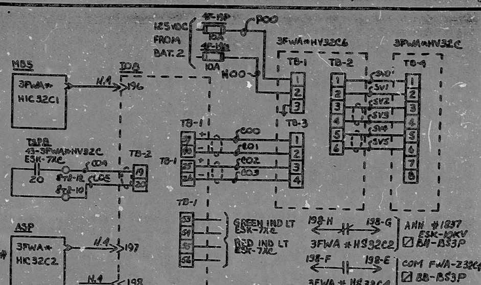
AUXILIARY FEEDWATER CONTROL VALVE [3FWA*HV32C] (C,P) CKT NO. 3FWAC11
