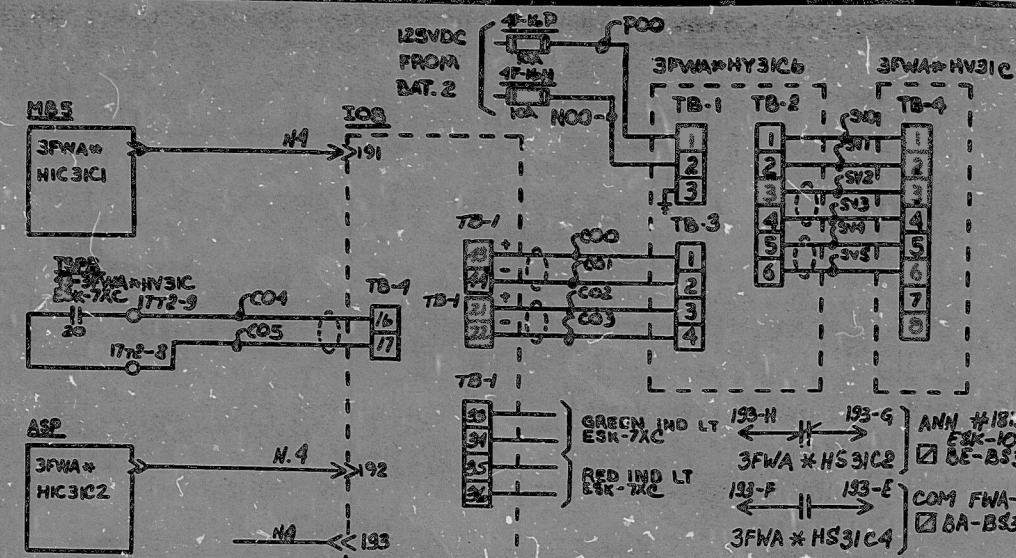
AUXILIARY FEEDWATER CONTROL VALVE [3FWA*HV31C] (C,P) CKT NO. 3FWAC10
