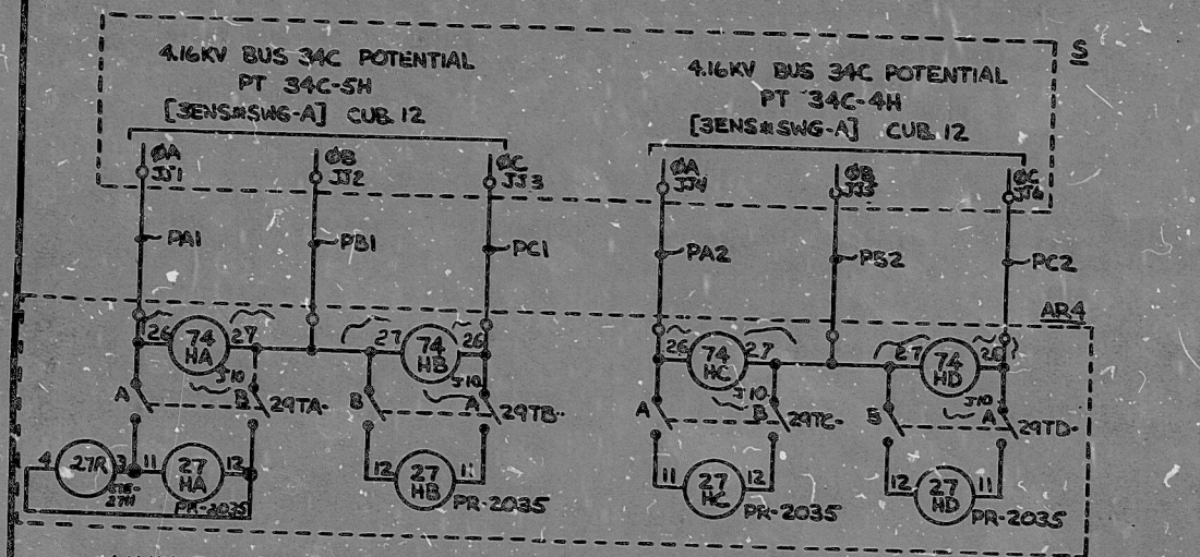
4.16KV BUS 34C [3ENS#SWG-A] UNDERVOLTAGE (HI SETPOINT) RELAYS CKT 3ENSA18(-O)
