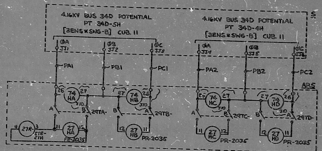
4.16KV BUS 34D [3ENS#SWG-B] UNDERVOLTAGE (HI SETPOINT) RELAYS CKT 3ENSB18(-P)
