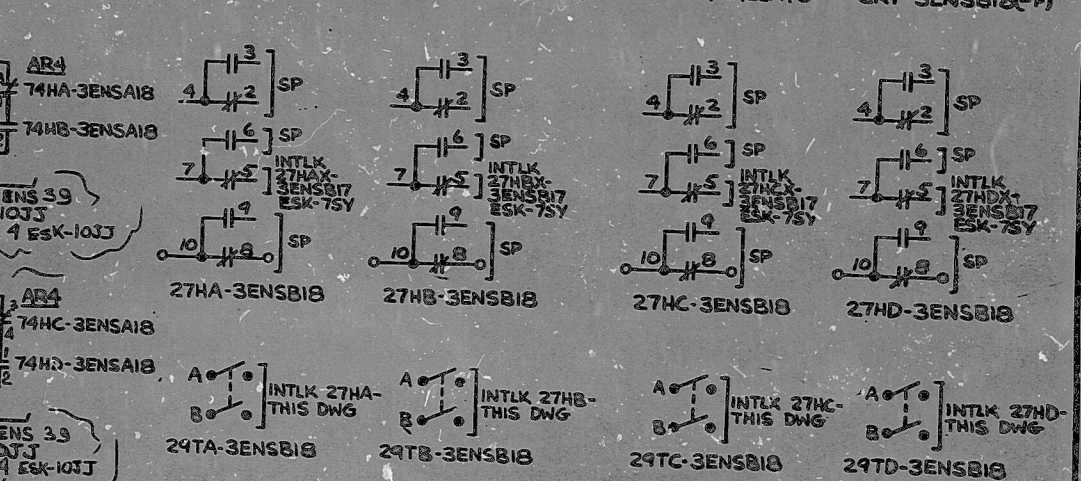
4.16KV BUS 34D [3ENS#SWG-B] UNDERVOLTAGE (HI SETPOINT) RELAYS CKT 3ENSB18(-P)
