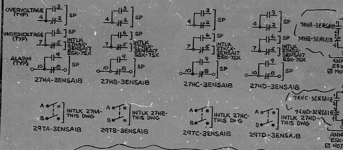
4.16KV BUS 34C [3ENS#SWG-A] UNDERVOLTAGE (HI SETPOINT) RELAYS CKT 3ENSA18(-O)
