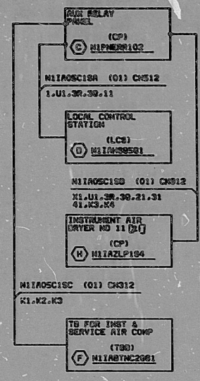
CABLE BLOCK DIAGRAM 1 SCHEMATIC NITROSC1 INSTRUMENT AIR DRYER BYPASS VALVE PV-8561
