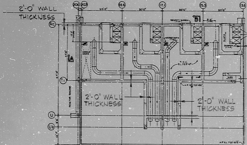
PLAN OF ELEV. 723'-0"
