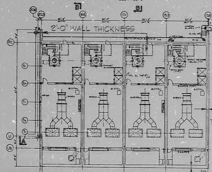
PLAN OF ELEV. 710'-9"
