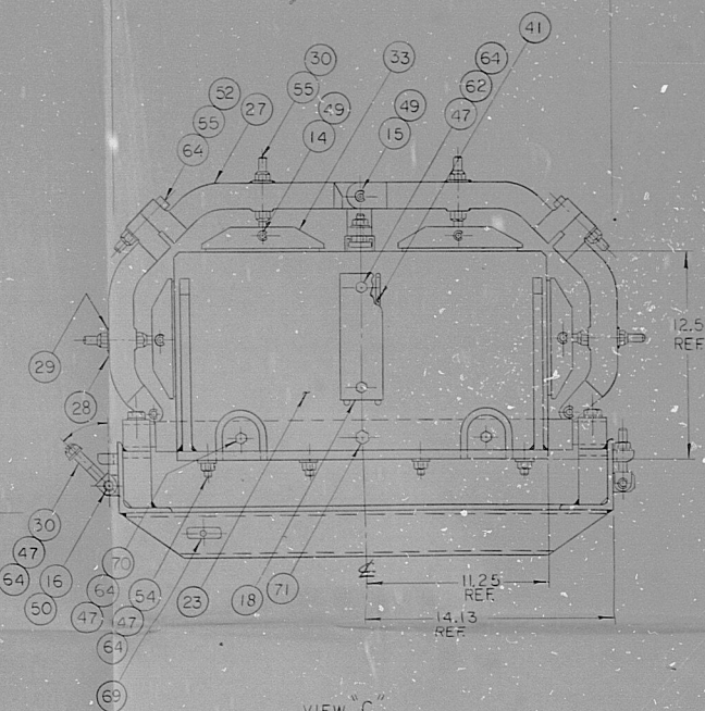
VIEW "C" SUPPORT FRAME ASSEMBLY ITEM (10)
