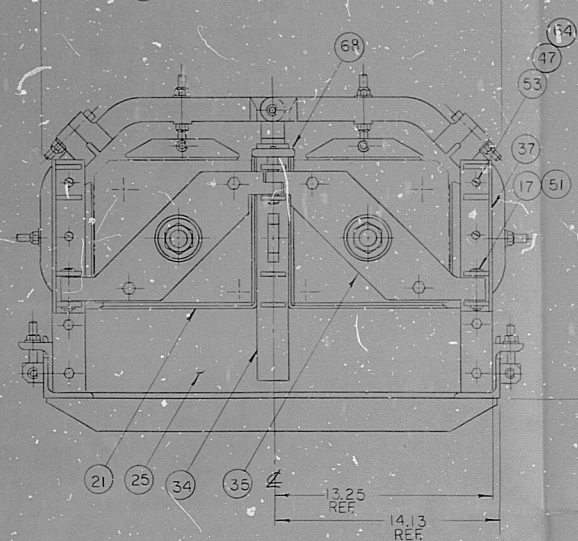
VIEW "D" TOP CLOSURE ASSEMBLY ITEM (12)
