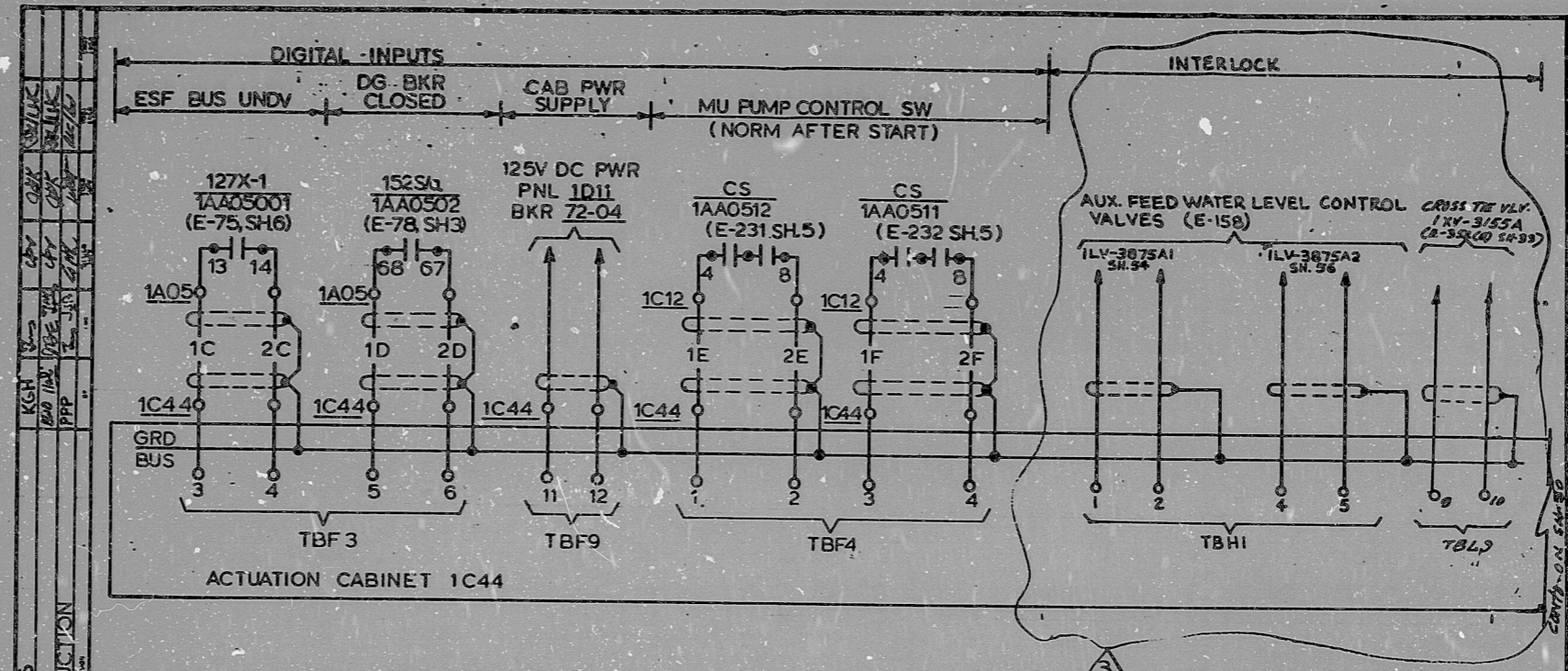
ACTUATION CABINET "A" INTERLOCKS SCHEME 1AQ403 SU DESIG 1-SAB
