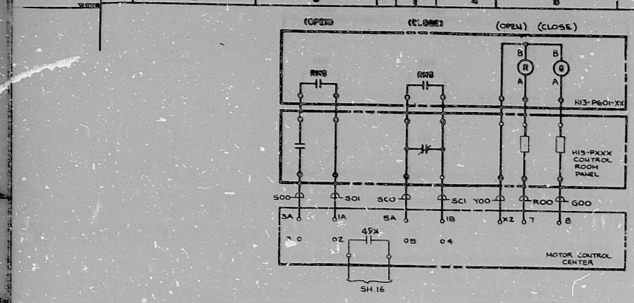
TYP FOR MOTOR OPERATED VALVES (REF 2.0) SEE S & W ESK-2L, 2M
