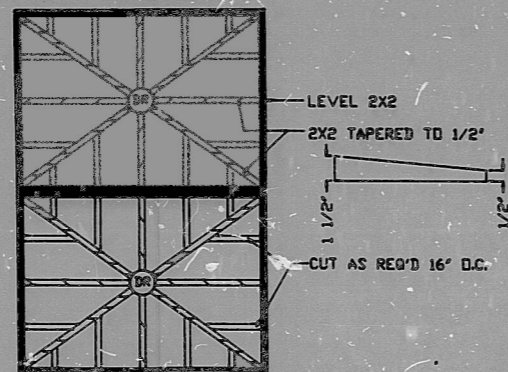
SHOWER FLOOR DETAIL SLOPED 4 DIRECTIONS TOWARDS SHOWER DRAIN 13 5/8"
