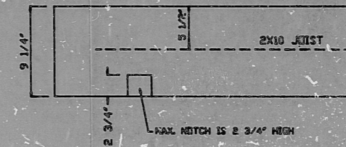
NOTCHING OF FLOOR JOIST
