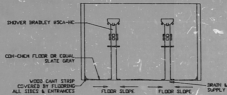
ELEVATION E-E
