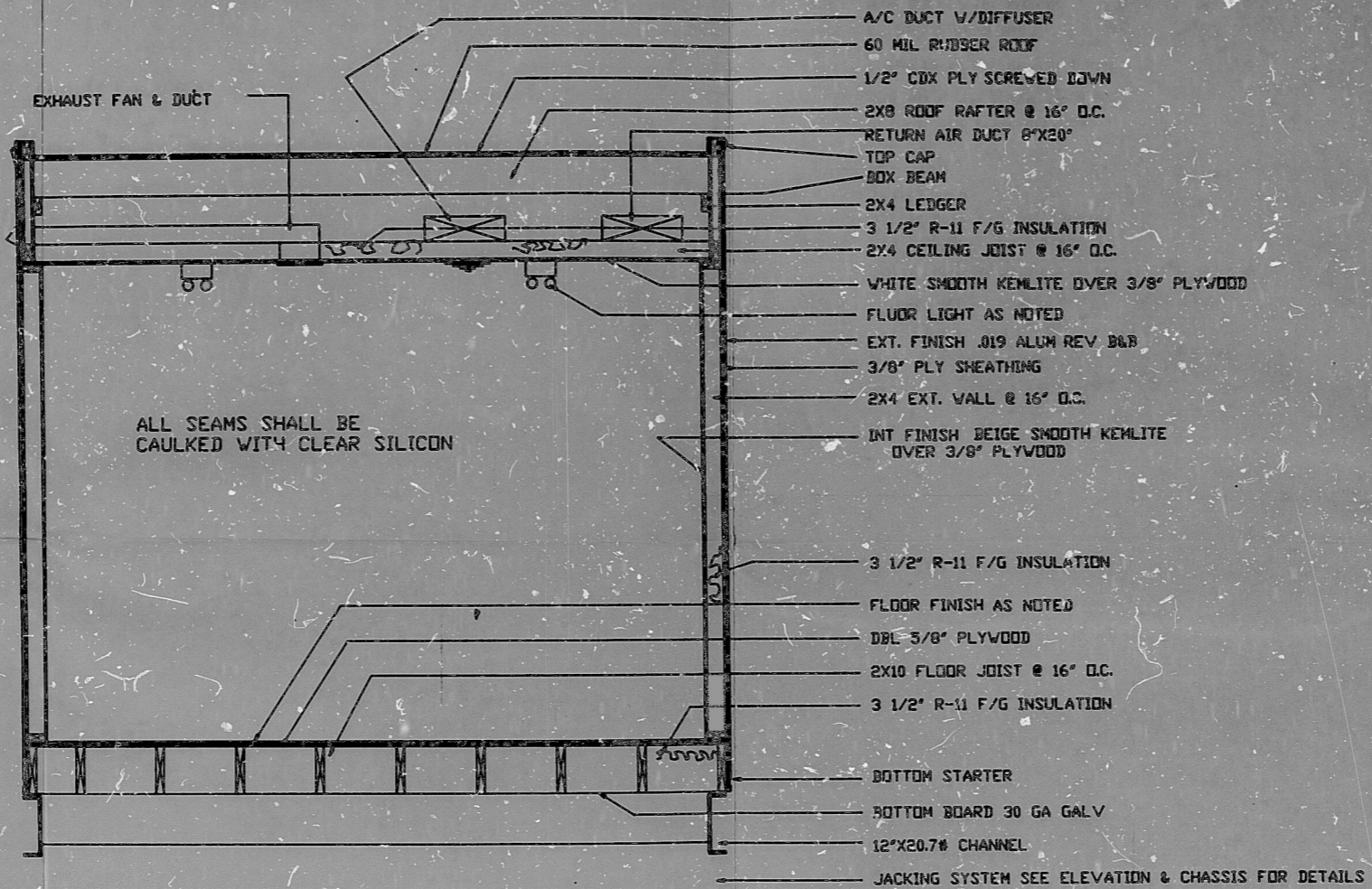
STD. CROSS SECTION
