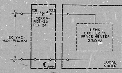
FIG. 3 H13-P634 RACK 1
