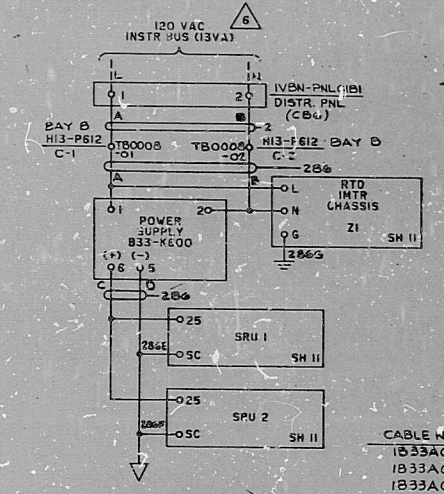
FIG. 12 H13-P612 PWR DISTRIBUTION
