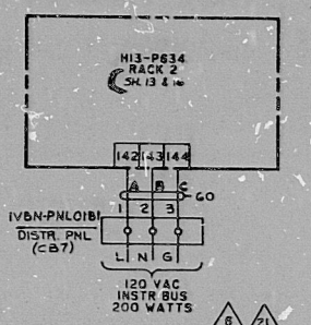
FIG. 4 H13-P634 RACK 2
