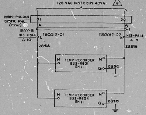
FIG. 2 H13-P614 AC POWER DISTRIBUTION
