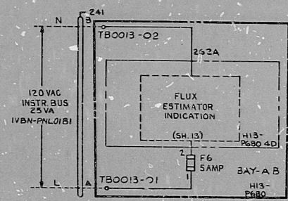
FIG. 5 POWER DISTRIBUTION
