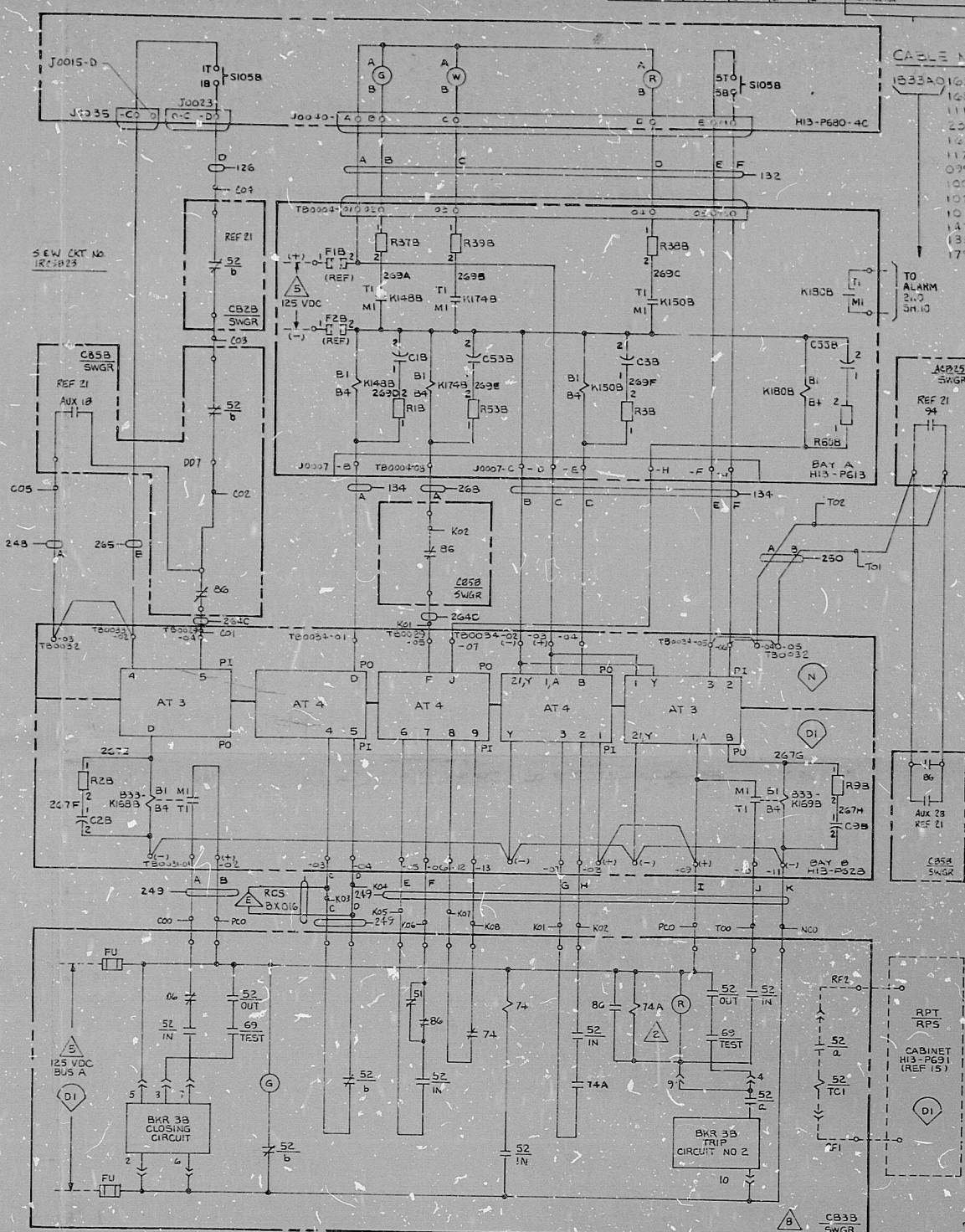
RECIRCULATION PUMP MOTOR C001B BREAKER 3B CONTROL (FOR DETAILS SEE S & W DWG ESK-5RC5041-5RC506) S & W. Ckt. No. 1R5B05
