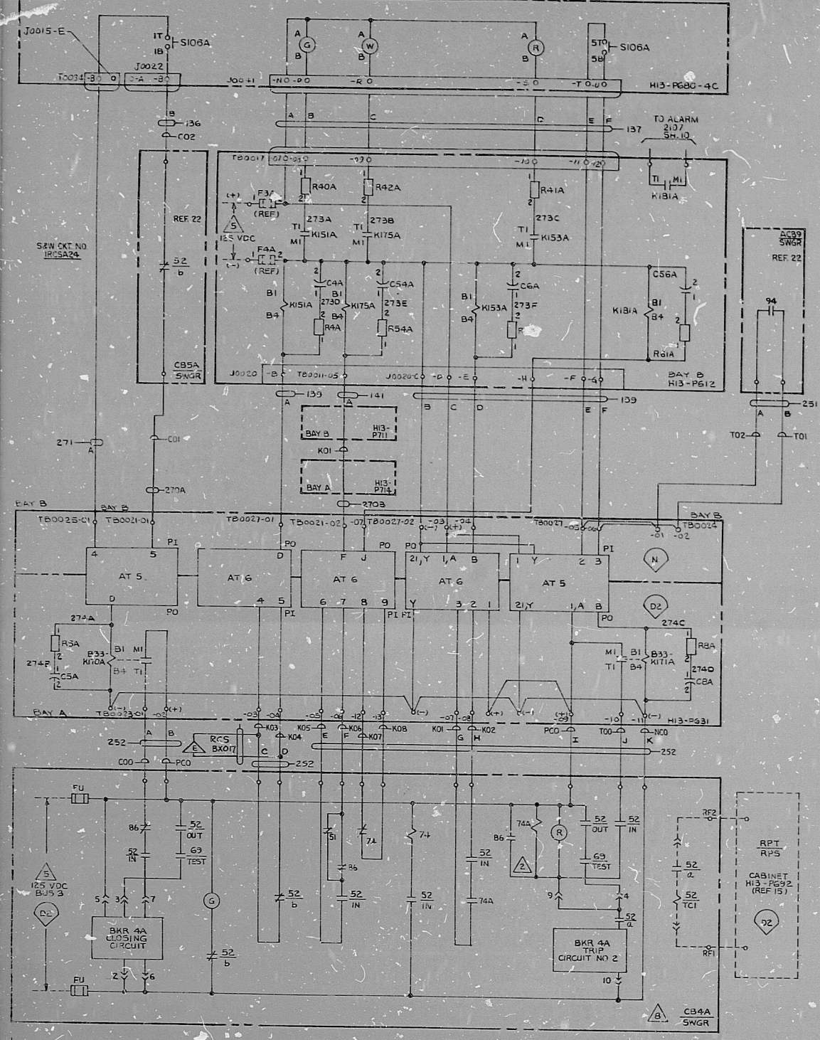
RECIRCULATION PUMP MOTOR C001A BREAKER 4A CONTROL (FOR DETAILS SEE S & W DWG ESK-SRC507 S&W CKT NO IRC5A24)
