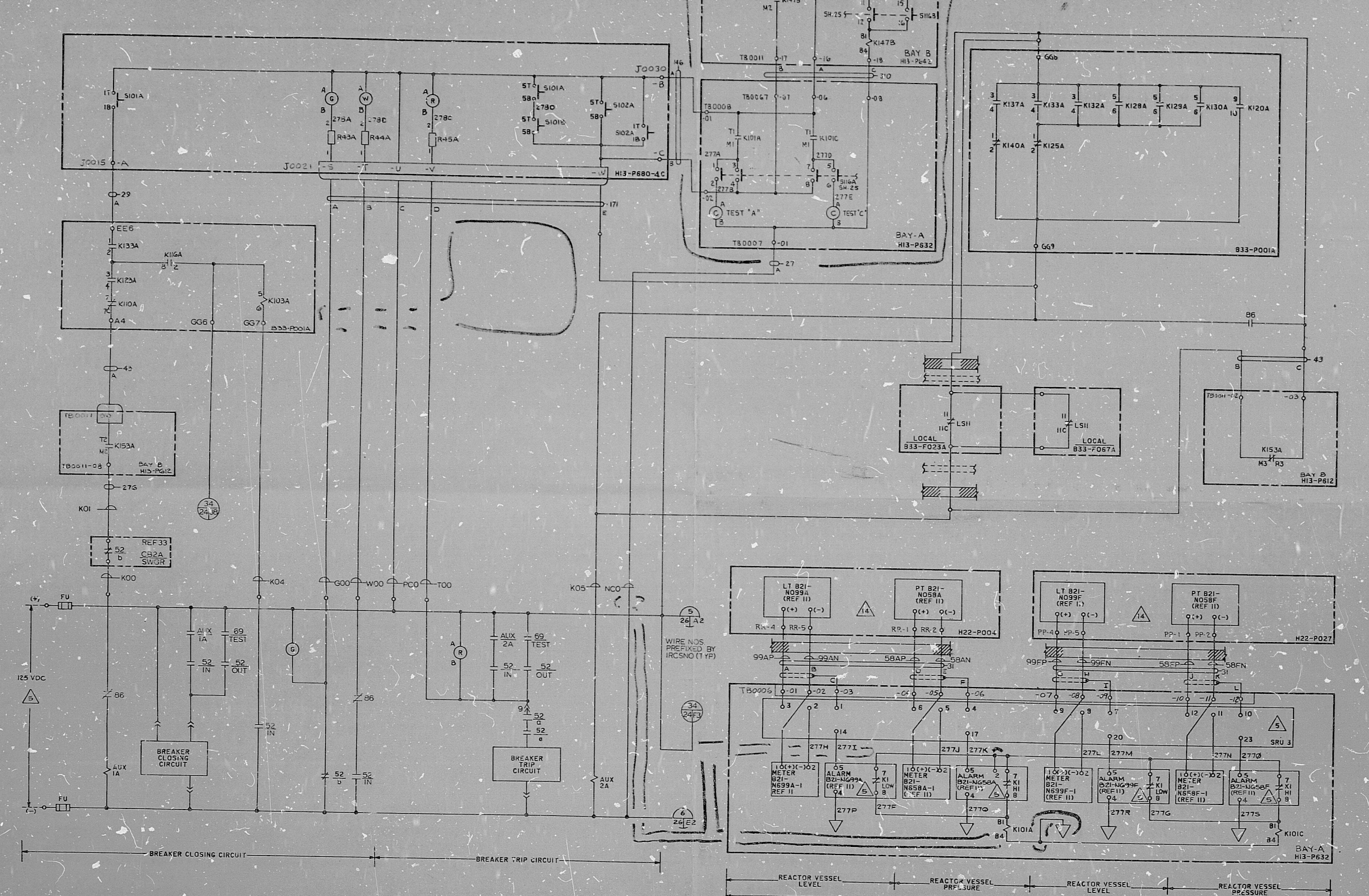
RECIRCULATION PUMP MOTOR COOLANT BREAKER SA CONTROL (FOR DETAILS SEE REF 31) SAW CRT NO. INPSA23
