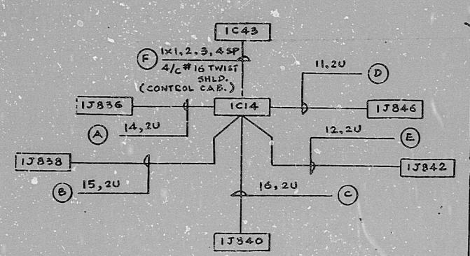
FOGG CIRCUIT FOR AUX. FEED WATER SYSTEM SCHEME NO. ICFW145 S.U. DESIG. later
