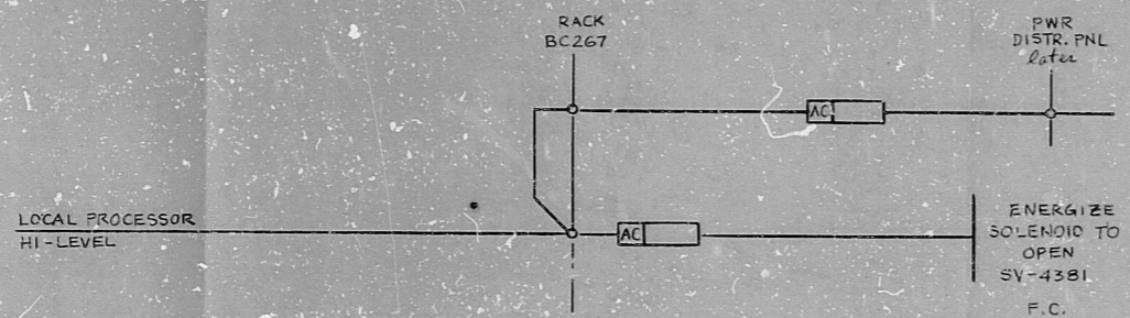
LOWER DRYWELL AIR COOLERS DRAIN SOLENOID VLV SV-4381
