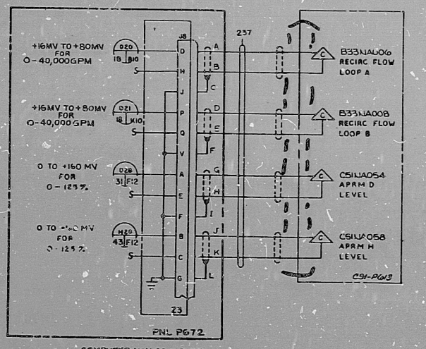
COMPUTER ANALOG INPUTS
