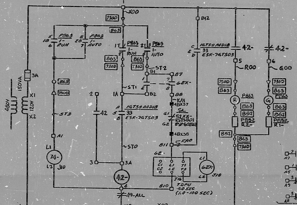
STBY GAS TRTMT DECAY HT REMOVAL FAN IGTS*FN2B CKT NO IGTS B03 LOCN. IEH5*MCC2D (BLUE)
