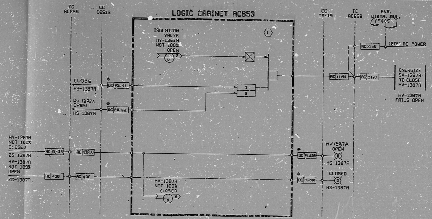
FWH NO. 5 EXTRACTION STEAM DRAIN ISOLATION VALVE HV-1387A
